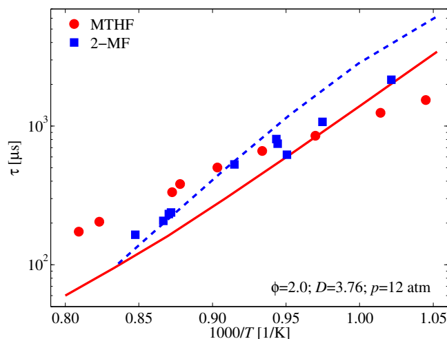
Figure 4.51: Ignition delay times of MTHF and 2-MF at an equivalence ratio of 2.0 and a nominal pressure of 12.0 atm. Model predictions: solid line is MTHF model by Moshhammer et al. [47] and dash line is 2-MF model by Somers et al. [12].
