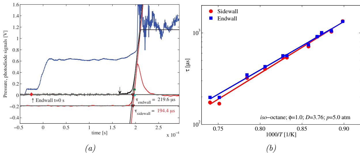
Figure 2.7: (a) Sidewall and endwall CH emission signals for stoichiometric iso-octane/ O_2 /Ar mixture at pressure of 5.0 atm, temperature of 1351 K, and D of 3.76. (b) Sidewall and endwall ignition delay time measurements for stoichiometric iso-octane/ O_2 /Ar mixture at pressure of 5.0 atm, and D of 3.76.
